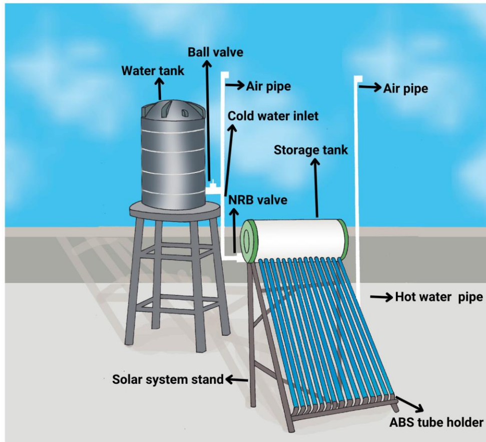
Fig 39: Evacuated Tubes Solar Heater and Components
