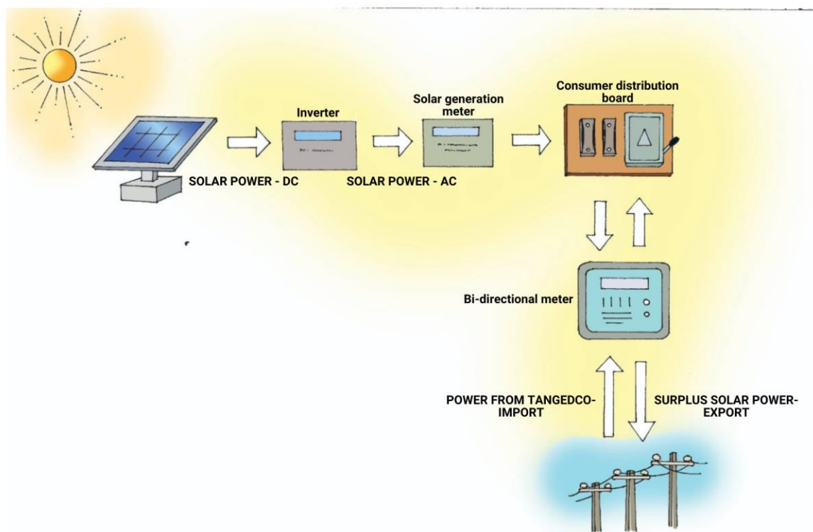
Fig 40: Working of Solar Rooftop Photovoltaic System
