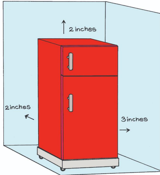
Fig 21: Refrigerator clearance space requirement
